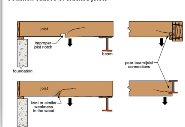
Common causes of cracked joists
