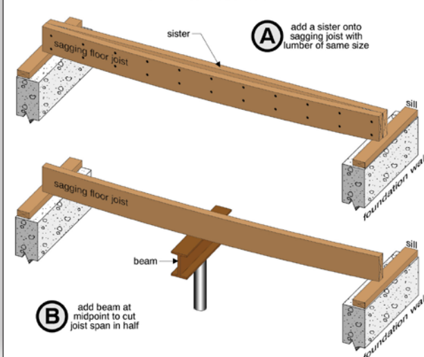
Two methods for improving sagging joists
