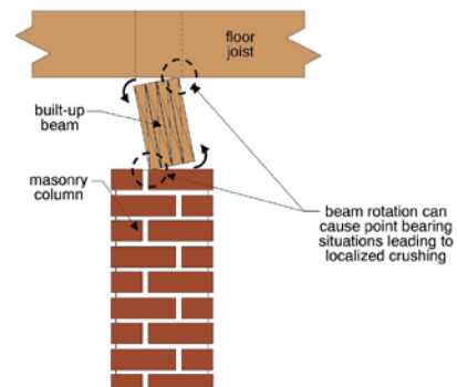
Rotated or twisted beams
