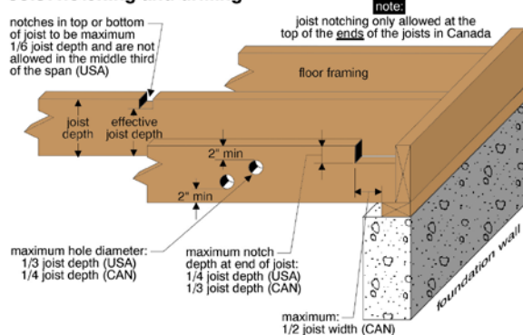
Joist notching and drilling
