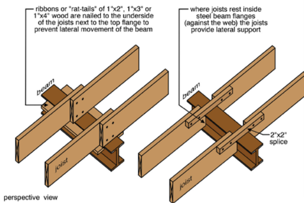
Lateral support for steel beams
