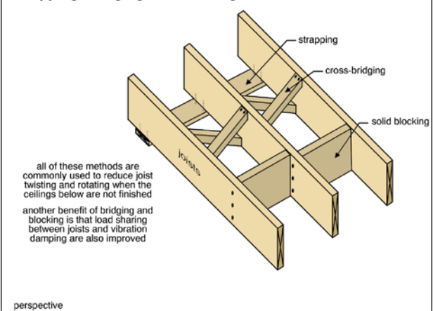
Strapping, bridging and blocking
