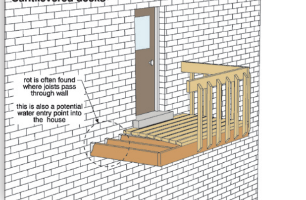
Cantilevered decks
