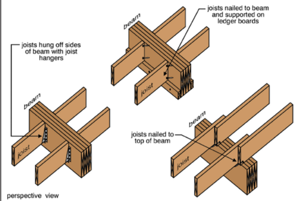
Lateral support for wood beams
